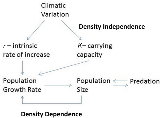
FIGURE 3-1 Population processes, including density-independent and density-dependent controls.
